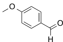
4-methoxybenzaldehyde
