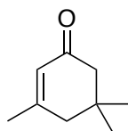
3,5,5-trimethyl-2-cyclohexen-1-one
